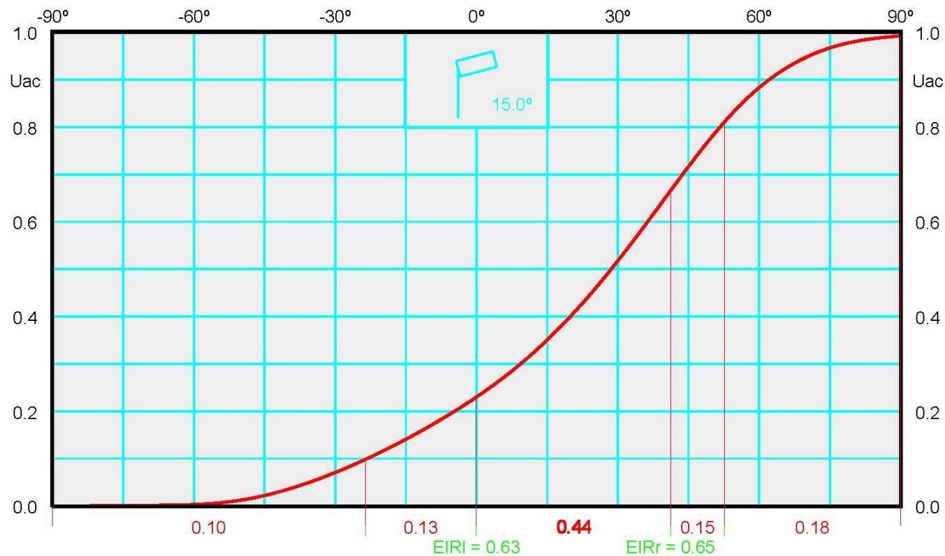
DIAGRAM OF ACCUMULATED UTILANCE / CIE 132:1999
