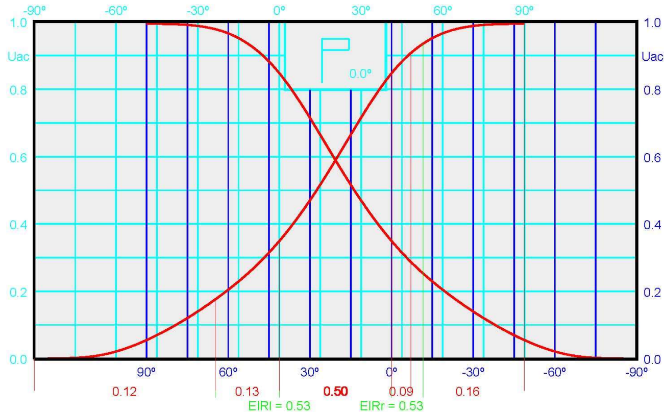
DIAGRAM OF ACCUMULATED UTILANCE / EN 13032-5
